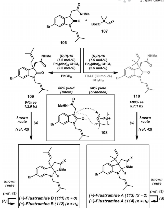
Scheme 15. Total syntheses of flustramides A and B and flustramines A and B. Reaction conditions: a) \text{AlH}_3\cdot\text{NMe}_2\text{Et} , THF, -15 °C (95% yield). b) \text{AlH}_3\cdot\text{NMe}_2\text{Et} , THF, room temp. (97% yield). c) \text{AlH}_3\cdot\text{NMe}_2\text{Et} , THF, -15 °C (92% yield). d) \text{AlH}_3\cdot\text{NMe}_2\text{Et} , THF, room temp. (90% yield).
