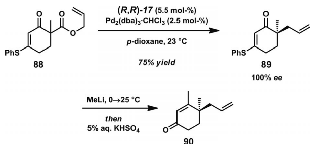
Scheme 12. Extension of \beta -keto ester substrate scope to vinylogous ester scaffolds.
