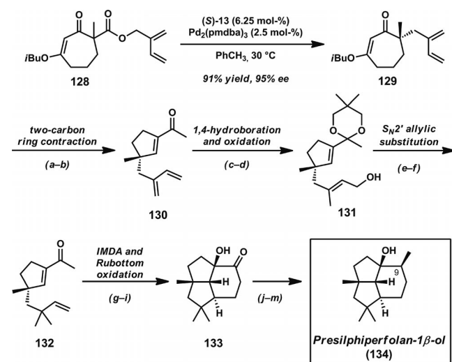
Scheme 18. Total synthesis of presilphiperfolan-1 \beta -ol. Reaction conditions: a) LiAlH 4 , Et 2 O, 0 °C (96% yield). b) LiOH, TFE, THF, 60 °C (96% yield). c) Neopentyl glycol, PPTS (5 mol-%), PhH, reflux (94% yield). d) HBPIn, Ni(cod) 2 (5 mol-%), PCy 3 (5 mol-%), PhCH 3 , 23 °C; then 3 M aq. NaOH, H 2 O 2 , THF, 0 → 23 °C (81% combined yield, 63% yield of desired linear isomer 131 ). e) Diethyl chlorophosphate, Et 3 N, DMAP (20 mol-%), CH 2 Cl 2 , 0 → 23 °C (84% yield). f) Zn(CH 3 ) 2 , CuCN (10 mol-%), THF, −78 → 23 °C; then 10% aq. HCl (94% yield). g) TBSOTf, Et 3 N, CH 2 Cl 2 , 0 → 23 °C (98% yield). h) p -Dioxane, 170 °C, sealed tube. i) DMDO, acetone, −78 °C; then TBAF, −78 → 23 °C (90% combined yield, two steps, 1:2 dr , 28% yield of desired diastereomer). j) KO t Bu, Ph 3 PCH 3 Br, THF, 0 → 23 °C (90% yield). k) HMDS, imidazole, TMSCl, CH 2 Cl 2 (96% yield). l) PtO 2 (5 mol-%), EtOAc, H 2 (1 atm). m) TBAF, THF, reflux (92% yield, two steps).
