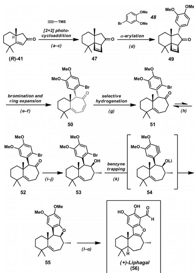
Scheme 8. Total synthesis of liphagal. Reaction conditions: a) TMS-acetylene, UV-B lamps, acetone. b) BF 3 ·OEt 2 , CH 2 Cl 2 . c) TBAF, THF (68% yield, three steps). d) [Pd(P( t Bu) 3 ) 2 ] (5 mol-%), 4-bromoveratrole, NaOtBu, THF, microwave irradiation, 120 °C (67% yield). e) Br 2 (1.8 equiv.), CHCl 3 (65% yield). f) Microwave irradiation, o -dichlorobenzene, 250 °C (68% yield). g) PtO 2 (20 mol-%), H 2 (1 atm), EtOAc (69% yield). h) NaOMe, MeOH, 65 °C (78% yield, three cycles). i) LDA, THF, –78 → 0 °C; then CH 3 I, –78 → 0 °C (68% yield). j) DIBAL, PhCH 3 (91% yield). k) LDA (3 equiv.), THF, –20 °C (83% yield). l) Pd/C (19 mol-%), H 2 (1 atm), EtOH, 21 °C (97% yield). m) NO + BF 4 – , CH 3 CN, 0 °C (70% yield). n) n BuLi, TMEDA, THF, 0 °C; then DMF, 0 → 21 °C (70% yield). o) BiI 3 , CH 2 Cl 2 (45% yield).
