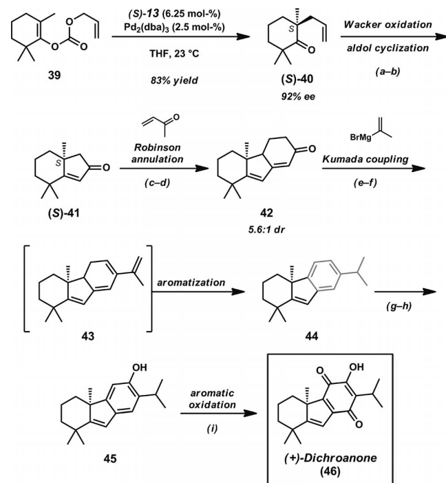
Scheme 7. Total synthesis of dichroanone. Reaction conditions : a) \text{PdCl}_2 (5 mol-%), \text{Cu}(\text{OAc})_2 \cdot \text{H}_2\text{O} (25 mol-%), \text{O}_2 (1 atm), DMA/ \text{H}_2\text{O} (7:1), 23 °C, Parr shaker (77% yield). b) \text{KOH} (0.45 equiv.), xylenes, 110 °C, Dean–Stark (96% yield). c) \text{LiHMDS} , THF, 0 \rightarrow 23 °C; then methyl vinyl ketone, –78 °C; then aq. \text{NH}_4\text{Cl} , –78 \rightarrow 23 °C (72% yield). d) Powdered \text{KOH} (2 equiv.), xylenes, 110 °C, Dean–Stark (80% yield). e) \text{LDA} , THF, –78 °C; then \text{PhN}(\text{Tf})_2 , –78 \rightarrow 23 °C. f) Isopropenylmagnesium bromide (2 equiv.), [\text{Pd}(\text{PPh}_3)_4] (5 mol-%), THF, 23 °C; then 6 M aq. \text{HCl} , 23 °C (65% yield, two steps). g) \text{Cl}_2\text{HCOCH}_3 , \text{TiCl}_4 , \text{CH}_2\text{Cl}_2 , –78 \rightarrow 23 °C (79% yield). h) Aq. \text{H}_2\text{O}_2 , aq. \text{H}_2\text{SO}_4 , THF/ \text{MeOH}/\text{H}_2\text{O} (2:5:1), 23 °C (74% yield). i) \text{IBX} (1.2 equiv.), \text{CHCl}_3 , 23 °C; then \text{C}_6\text{F}_5\text{SH} (4 equiv.), 23 °C; then \text{O}_2 (1 atm), \text{NaOH} (10 equiv.), \text{MeOH} , 23 \rightarrow 75 °C; then 6 M aq. \text{HCl} , 23 °C (35% yield).
