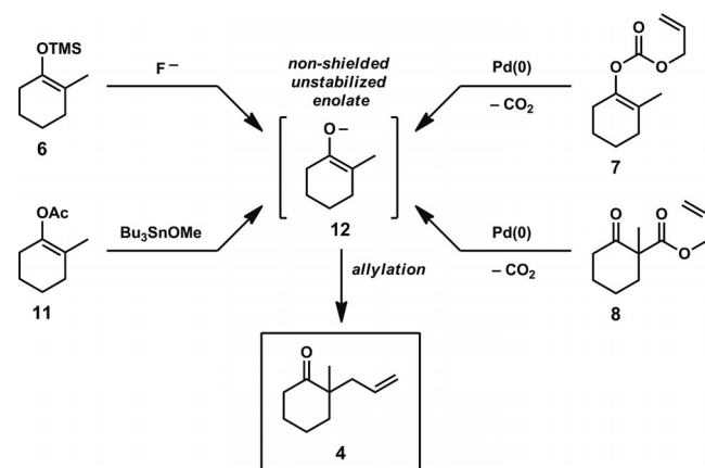
Scheme 3. Tsuji reactions for the allylation of non-shielded, non-stabilized enolates.
