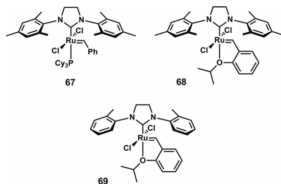
Figure 3. Ruthenium olefin metathesis catalysts.
