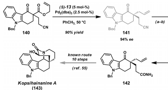
Scheme 20. Formal synthesis of kopsihainanine A. Reaction conditions: a) HCO 2 H, b) K 2 CO 3 , BnBr, acetone, 55 °C (94% yield, two steps).
