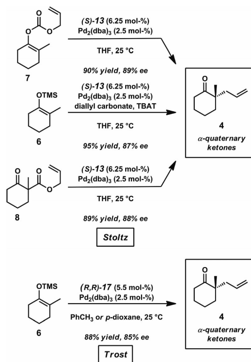
Scheme 4. Pd-catalyzed asymmetric allylic alkylation reactions with allyl enol carbonate, silyl enol ether, and \beta -keto ester substrate classes.
