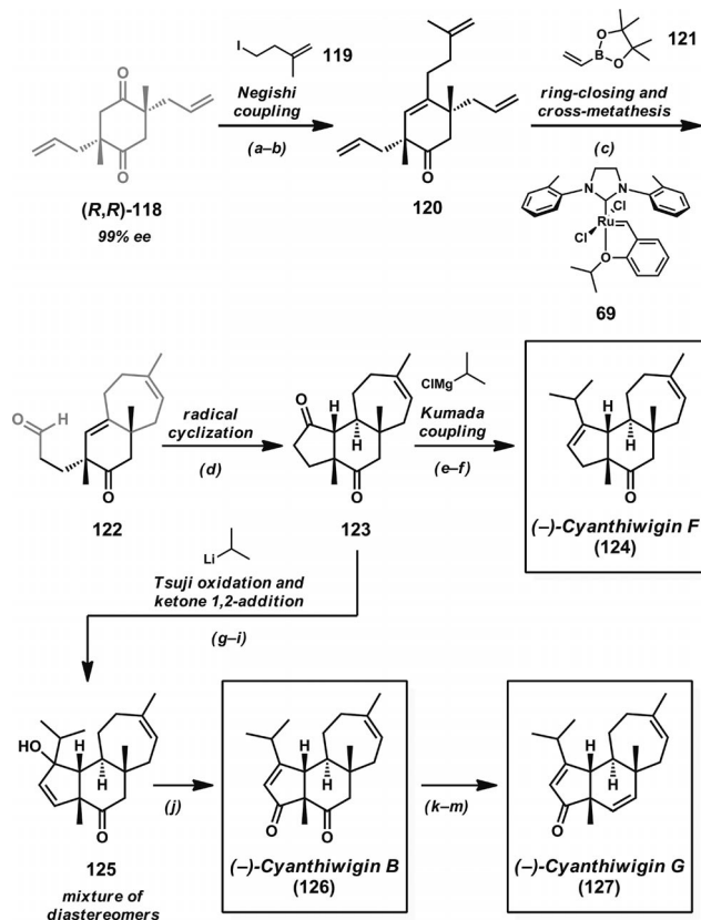
Scheme 17. Total syntheses of cyanthiwiggins B, F, and G. Reaction conditions: a) KHMDS, PhN(Tf) 2 , THF, −78 °C (73% yield). b) Zn(0), TMSCl, 1,2-dibromoethane, alkyl iodide 119 , THF, 65 °C; then [Pd(PPh 3 ) 4 ] (5 mol-%) (78% yield). c) Vinylboronic ester 121 , Grubbs–Hoveyda third-generation catalyst ( 69 , 10 mol-%), PhH, 60 °C; then NaBO 3 , THF/H 2 O (51% yield). d) t BuSH, AIBN, PhH, 80 °C. e) KHMDS, PhN(Tf) 2 , THF, −78 °C (60% yield). f) i PrMgCl, CuCN, THF; [Pd(dppf)Cl 2 ] (10 mol-%) (41% yield). g) KHMDS, THF −78 °C; then allyl chloroformate. h) [Pd 2 (pmdba) 3 ] (5 mol-%), CH 3 CN, 80 °C (57% yield, two steps). i) CeCl 3 , i PrLi, THF, −78 °C (76% yield, mixture of diastereomers). j) PCC, CH 2 Cl 2 (86% yield). k) NaBH 4 , MeOH/CH 2 Cl 2 , 25 °C. l) MnO 2 , CH 2 Cl 2 (15% yield, two steps). m) Martin's sulfuran, CDCl 3 (48% yield).
