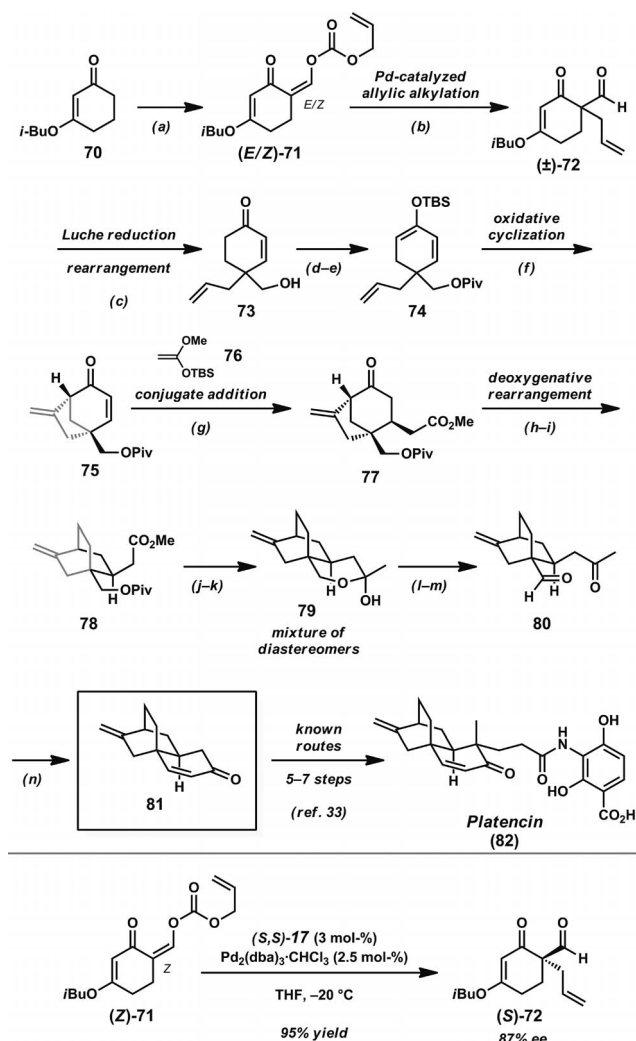
Scheme 10. Formal synthesis of ( \pm )-platencin. Reaction conditions: a) NaH, \text{HCO}_2\text{iBu} , 0 °C; then \text{ClCO}_2\text{allyl} , cat. KH, THF, 0 °C. b) \text{Pd}(\text{OAc})_2 (1.3 mol-%), \text{PPh}_3 , THF, 20 °C (92% yield, two steps). c) \text{NaBH}_4 , \text{CeCl}_3 \cdot 7\text{H}_2\text{O} , MeOH, 0 °C; then p\text{TSA} , \text{H}_2\text{O}/\text{Et}_2\text{O} , room temp. d) \text{PivCl} (2 equiv.), pyridine (4 equiv.), DMAP (0.05 equiv.), \text{CH}_2\text{Cl}_2 , room temp. (94% yield, two steps). e) LDA (1.5 equiv.), TBSCl (2 equiv.), HMPA (1 equiv.), THF, -80 °C \rightarrow r.t. (88% yield). f) \text{O}_2 , \text{Pd}(\text{OAc})_2 (5.8 mol-%), DMSO (85% yield). g) \text{H}_2\text{C}=\text{C}(\text{OMe})\text{OTBS} ( 76 , 1.5 equiv.), \text{TiCl}_4 (1.2 equiv.), \text{CH}_2\text{Cl}_2 , -80 °C (88% yield). h) \text{TsNHNH}_2 (1.3 equiv.), MeOH, 60 °C (95% yield). i) \text{NaCNBH}_3 , \text{ZnCl}_2 , MeOH, 60 °C (60% yield). j) \text{HCl} \cdot \text{NH}(\text{OMe})\text{Me} (6 equiv.), \text{Me}_3\text{Al} (5 equiv.), \text{CH}_2\text{Cl}_2 , 0 °C. k) \text{MeLi} (6 equiv.), \text{Et}_2\text{O} , -80 \rightarrow -30 °C. l) \text{LiAlH}_4 (1 equiv.), \text{Et}_2\text{O} , -80 \rightarrow 0 °C (85% yield, two steps). m) (\text{COCl})_2 (5.8 equiv.), DMSO (9 equiv.), -80 °C, \text{Et}_3\text{N} (73% yield). n) NaOH (6.5 equiv.), EtOH, 20 °C, 20 h (87% yield).
