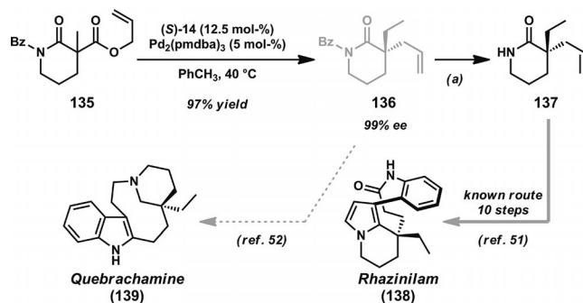
Scheme 19. Formal synthesis of rhazinilam and synthetic approach to quebrachamine. Reaction conditions: a) LiOH·H 2 O, MeOH, 23 °C (96% yield).
