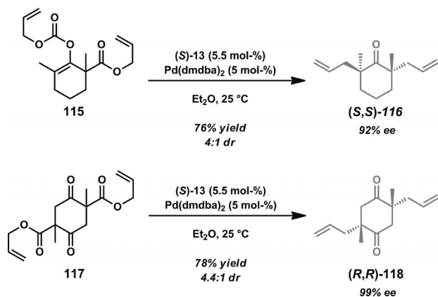
Scheme 16. Double enantioselective decarboxylative allylic alkylation reactions.
