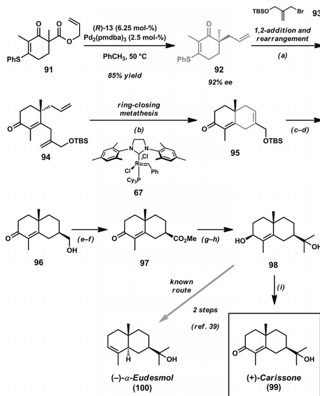
Scheme 13. Total synthesis of carissone and formal synthesis of \alpha -eudesmol. Reaction conditions: a) allylic bromide 93 , Mg(0), \text{I}_2 , 0 \rightarrow 23 ^\circ\text{C} (94% yield). b) Grubbs second-generation catalyst ( 67 , 3 mol-%), PhH, 40 ^\circ\text{C} (99% yield). c) Rh/ \text{Al}_2\text{O}_3 (5 mol-%), \text{H}_2 (1 atm), MeOH. d) HCl, THF (56% yield, two steps). e) Dess–Martin periodinane, \text{CH}_2\text{Cl}_2 , 0 \rightarrow 23 ^\circ\text{C} . f) \text{NaClO}_2 , \text{NaH}_2\text{PO}_4 , 2-methylbut-2-ene, t BuOH/ \text{H}_2\text{O} ; then \text{CH}_2\text{N}_2 (87% yield, two steps). g) \text{CeCl}_3 \cdot 7\text{H}_2\text{O} , \text{NaBH}_4 , MeOH, -45\text{ }^\circ\text{C} . h) MeMgBr, THF, 0 \rightarrow 26 ^\circ\text{C} (73% yield, two steps). i) \text{MnO}_2 , 4 \text{\AA} MS, \text{CH}_2\text{Cl}_2 (100% yield).
