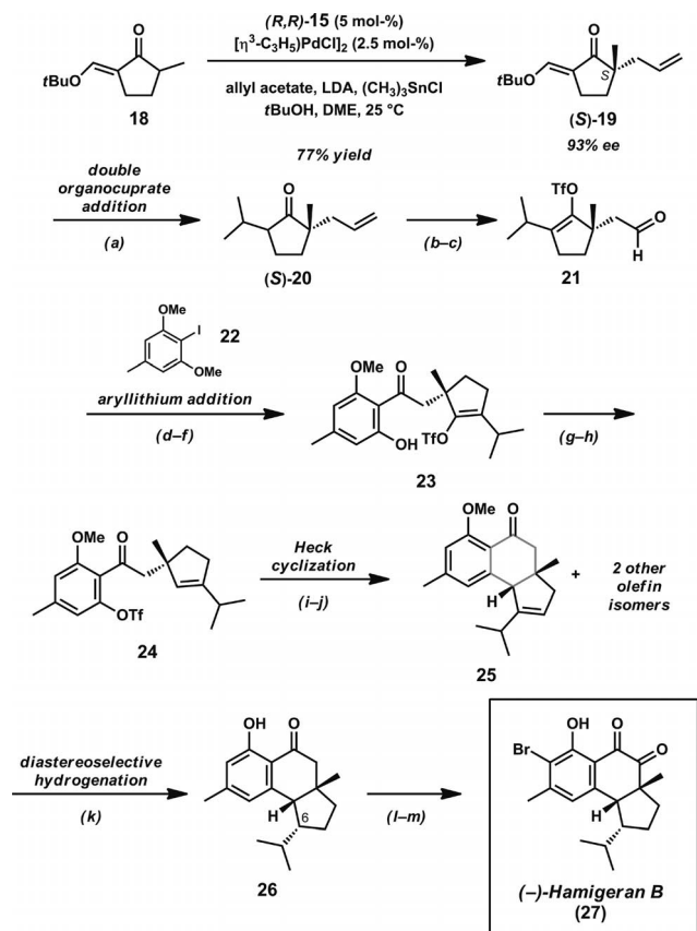
Scheme 5. Total synthesis of hamigeran B. Reaction conditions: a) (\text{CH}_3)_2\text{CuLi} , \text{Et}_2\text{O} , -20^\circ\text{C} (89% yield). b) LDA, THF, -78 \rightarrow 0^\circ\text{C} ; then \text{PhN}(\text{Tf})_2 (87% yield). c) \text{OsO}_4 (3.77 mol-%), NMO, THF, \text{H}_2\text{O} ; then \text{NaIO}_4 . d) Iodoarene 22 , DME, -55^\circ\text{C} ; then aldehyde 21 . e) Dess–Martin periodinane, \text{NaHCO}_3 , \text{CH}_2\text{Cl}_2 , 75% yield (three steps). f) \text{BCl}_3 , \text{CH}_2\text{Cl}_2 , -20^\circ\text{C} (85% yield). g) \text{Pd}(\text{OAc})_2 (10 mol-%), dppf (20 mol-%), \text{HCO}_2\text{H} , \text{Et}_3\text{N} , DMF, 70^\circ\text{C} (94% yield). h) \text{TiF}_2\text{O} , \text{CH}_2\text{Cl}_2 , pyridine, 0^\circ\text{C} (94% yield). i) \text{Pd}(\text{OAc})_2 , dppb, \text{K}_2\text{CO}_3 , \text{PhCH}_3 . j) \text{BBr}_3 , \text{CH}_2\text{Cl}_2 , -78^\circ\text{C} (51% yield, two steps). k) Ir black, \text{H}_2 (1500 psi), \text{EtOH} (>99% yield). l) \text{SeO}_2 , cat. \text{AcOH} , p -dioxane (90% yield). m) NBS, i\text{Pr}_2\text{NH} (5 mol-%), \text{CH}_2\text{Cl}_2 (85% yield).
