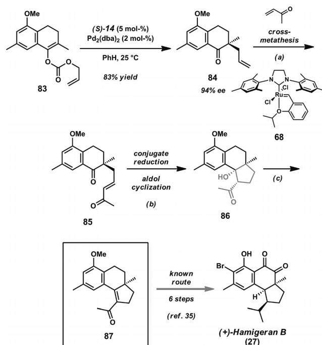
Scheme 11. Formal synthesis of hamigeran B. Reaction conditions: a) methyl vinyl ketone (10 equiv.), Grubbs-Hoveyda second-generation catalyst ( 68 , 10 mol-%), PhH, 35 °C (66% yield). b) [\text{Ph}_3\text{PCuH}]_6 (0.5 equiv.), \text{PhCH}_3 , -40 °C. c) \text{SOCl}_2 (15 equiv.), DMAP (30 mol-%), pyridine, 0 °C (62% yield).
