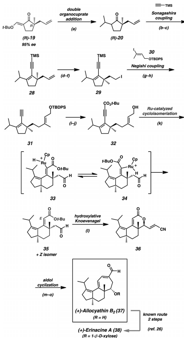
Scheme 6. Total synthesis of allocyathin B 2 . Reaction conditions: a) (\text{CH}_3)_2\text{CuLi} , \text{Et}_2\text{O} , -20^\circ\text{C} (89% yield). b) LDA, THF, -78 \rightarrow 0^\circ\text{C} ; then \text{PhN}(\text{Tf})_2 (96% yield). c) [\text{Pd}_2(\text{dba})_3]\cdot\text{CHCl}_3 (2.5 mol-%), \text{PPh}_3 (20 mol-%), \text{CuI} (5 mol-%), TMS-acetylene, n\text{BuNH}_2 , 50^\circ\text{C} (85% yield). d) \text{OsO}_4 (1 mol-%), NMO; then \text{NaIO}_4 (87% yield). e) \text{NaBH}_4 , MeOH (94% yield). f) \text{PPh}_3 , \text{I}_2 , imidazole (97% yield). g) t\text{BuLi} , \text{ZnCl}_2 , THF, -78^\circ\text{C} \rightarrow \text{r.t.} ; then [\text{Pd}(\text{PPh}_3)_4] (5 mol-%), vinyl iodide 30 . h) \text{K}_2\text{CO}_3 , MeOH (74% yield, two steps). i) n\text{BuLi} , THF, -78^\circ\text{C} ; then \text{Boc}_2\text{O} , -78 \rightarrow \text{r.t.} (99% yield). j) TBAF, THF (52–55% yield). k) \text{CpRu}(\text{CH}_3\text{CN})_3\text{PF}_6 (20 mol-%), DMF (1 equiv.), butan-2-one, room temp. (48% yield of 35 , or 55% combined yield, 6.7:1 E/Z ratio). l) \text{PhS}(\text{O})\text{CH}_2\text{CN} , piperidine, \text{PhH} (75% yield). m) \text{Pd/C} (10%), \text{EtOAc} , \text{H}_2 (1 atm) (83% yield). n) DIBAL, \text{CH}_2\text{Cl}_2 , -78^\circ\text{C} . o) KOH, MeOH, 60^\circ\text{C} (51% yield, two steps).
