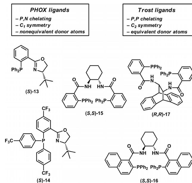
Figure 2. Selected chiral ligands for Pd-catalyzed asymmetric allylic alkylation reactions.
