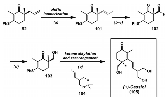
Scheme 14. Total synthesis of cassiol. Reaction conditions: a) [\text{PdCl}_2(\text{CH}_3\text{CN})_2] (10 mol-%), PhH, 60 °C (99% yield, 13:1 ratio 101/92 ). b) \text{OsO}_4 (10 mol-%), DABCO, \text{K}_3\text{Fe}(\text{CN})_6 , \text{K}_2\text{CO}_3 , t\text{BuOH}/\text{H}_2\text{O} (1:1), 35 °C. c) \text{Pb}(\text{OAc})_4 , PhH, 30 °C (70% yield). d) \text{Li}(\text{O}t\text{Bu})_3\text{AlH} , THF, 0 °C (85% yield). e) Vinyl iodide 104 , t\text{BuLi} , \text{Et}_2\text{O} , -78 °C; then vinylogous thioester 103 ; then aq. HCl, TBME (36% yield).
