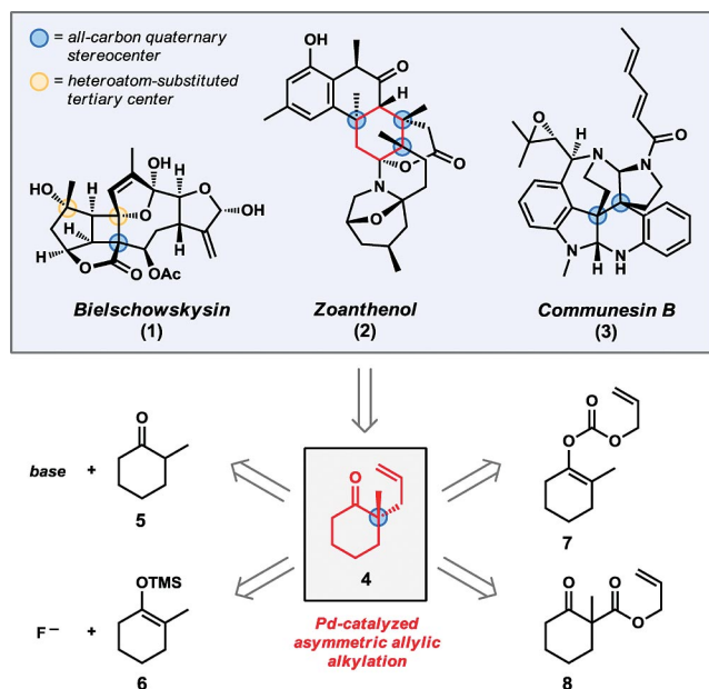
Figure 1. Natural products as an inspiration for the development of asymmetric catalysis.
