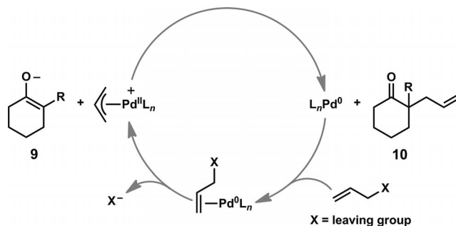
Scheme 1. General mechanism for Pd-catalyzed allylic alkylation reactions.
