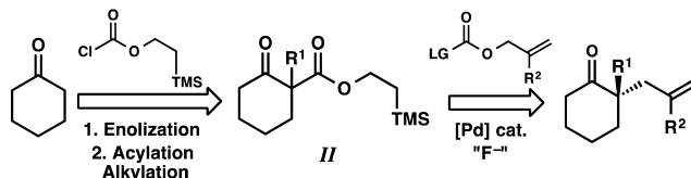
Figure 1. New substrate design enables broader functional group ( R^2 ) scope in allylic alkylation reactions.
