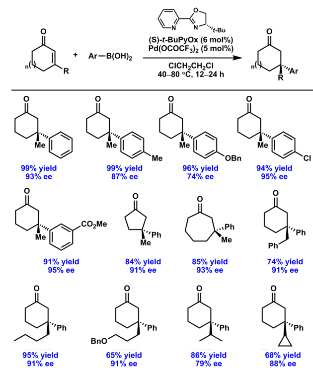
Scheme 3. Large Scale Conjugate Additions
