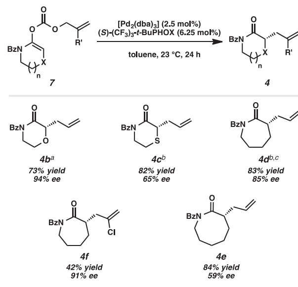
Scheme 3. Substrate scope of enol carbonates. Reaction conditions: A mixture of 7 (0.20 mmol), \text{Pd}_2(\text{dba})_3 (0.005 mmol), and (S)\text{-(CF}_3)_3\text{-t-BuPHOX} (0.0125 mmol) in toluene (0.033 M) was stirred at 23 °C for 24 h. Yield was isolated yield and enantiomeric excess was determined by chiral SFC analysis. a Performed at 50 °C. b Performed at 40 °C. [ \text{Pd}_2(\text{pmdba})_3 ] was used as a catalyst.
