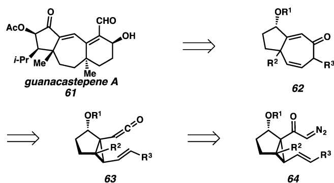
Scheme 13. Synthetic inspiration for the tandem Wolff–Cope rearrangement.
