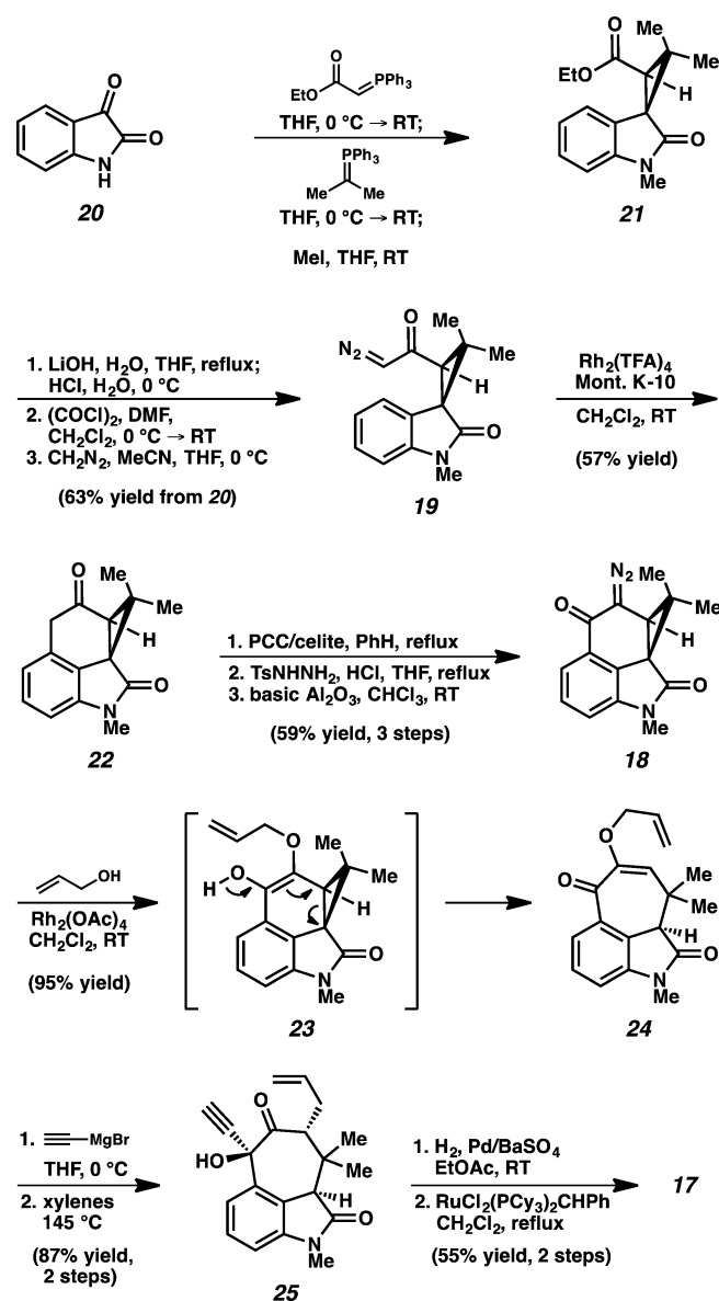
Scheme 5. Synthesis of the carbon skeleton of N -methylwelwitindolinone C isothiocyanate.
