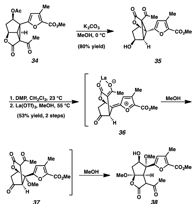
Scheme 8. Cyclopropane fragmentation.
