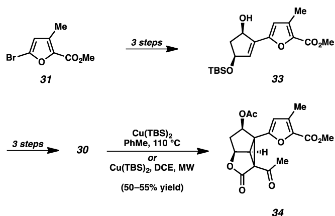
Scheme 7. Synthesis of donor–acceptor cyclopropane 34 . \text{Cu}(\text{TBS})_2 = bis( N - tert -butylsilylaldiminato)copper(II).
