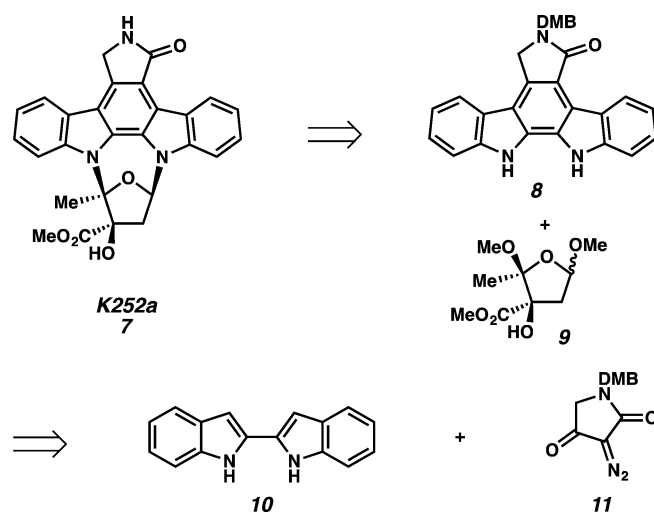
Scheme 2. Retrosynthetic analysis of K252a.
