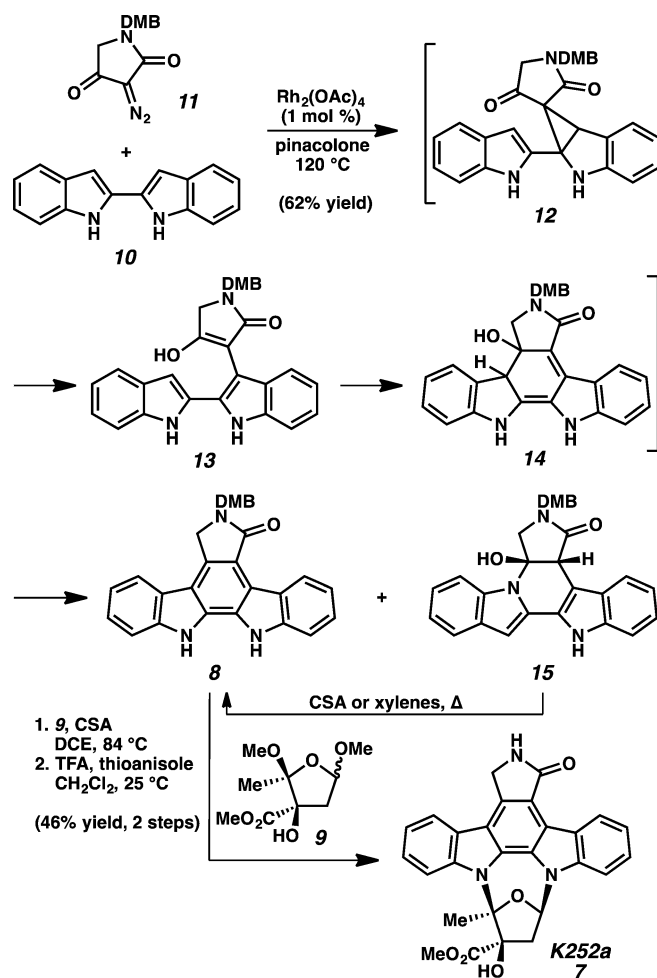
Scheme 3. Total synthesis of K252a.
