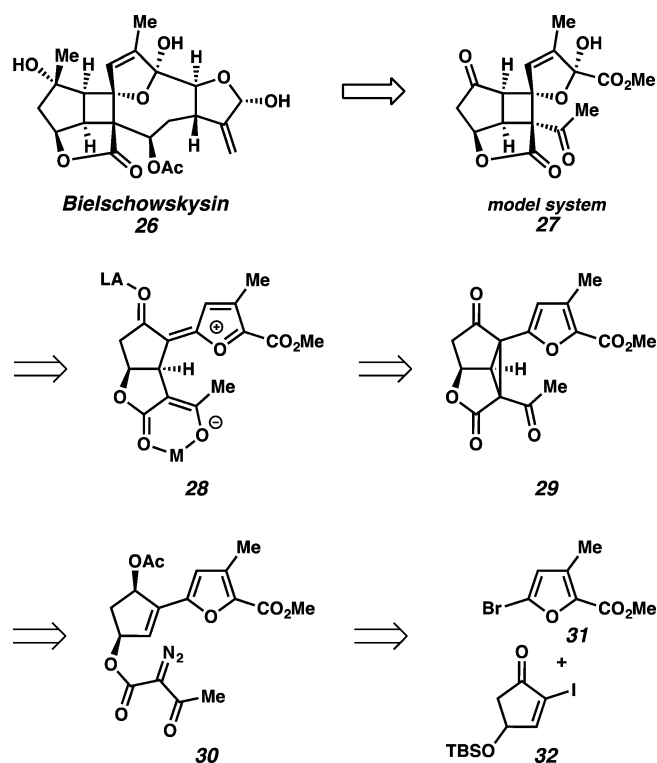
Scheme 6. Retrosynthetic analysis of bielschowskysin.
