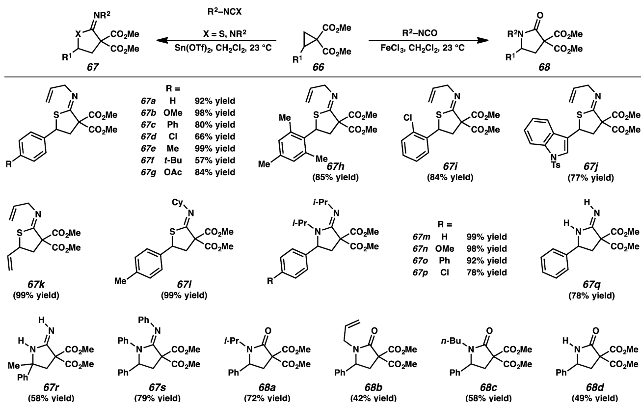
Scheme 15. Selected scope of cycloadditions of donor–acceptor cyclopropanes with heterocumulenes.
