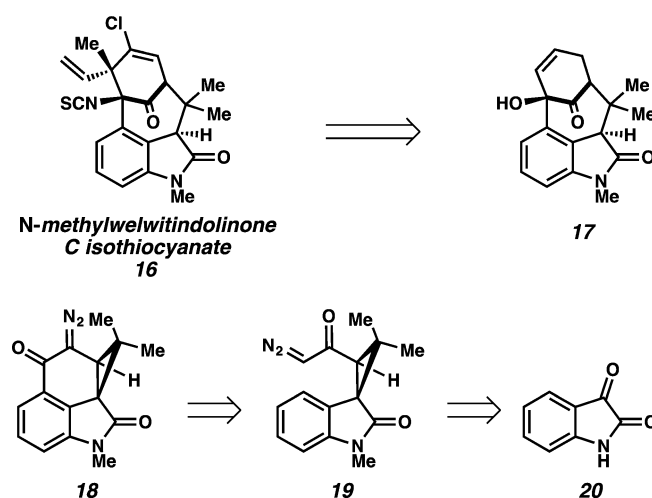
Scheme 4. Retrosynthetic analysis of N -methylwelwitindolinone C isothiocyanate.
