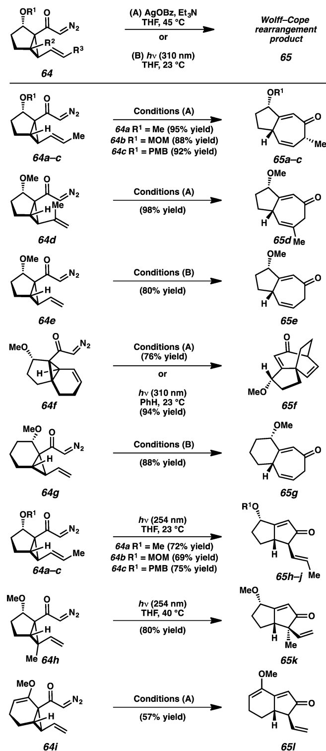
Scheme 14. Selected scope of the tandem Wolff-Cope rearrangement.
