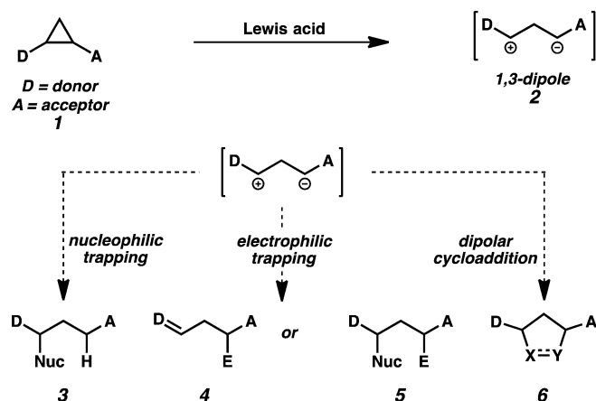
Scheme 1. Reactivity modes of donor–acceptor cyclopropanes.
