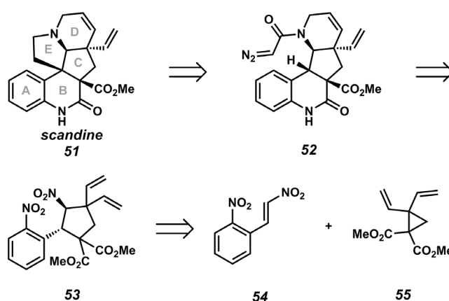
Scheme 11. Retrosynthetic analysis of scandine.
