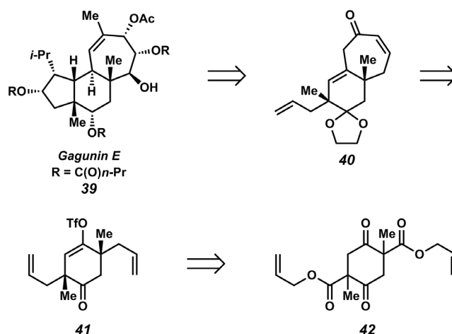
Scheme 9. Retrosynthetic analysis of gagunin E.
