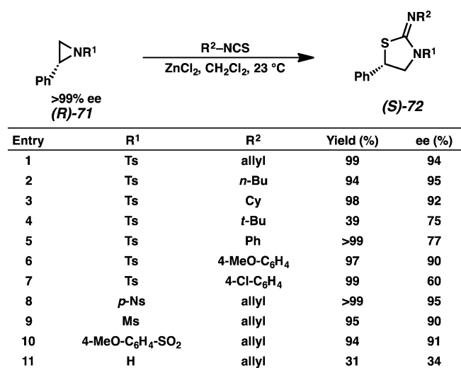
Scheme 18. Scope of the stereoselective cycloaddition of activated aziridines with heterocumulenes.
