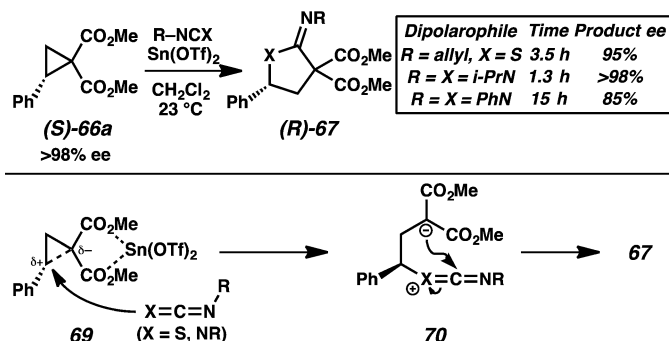
Scheme 16. Proposed mechanism of cyclopropane-heterocumulene cycloadditions.
