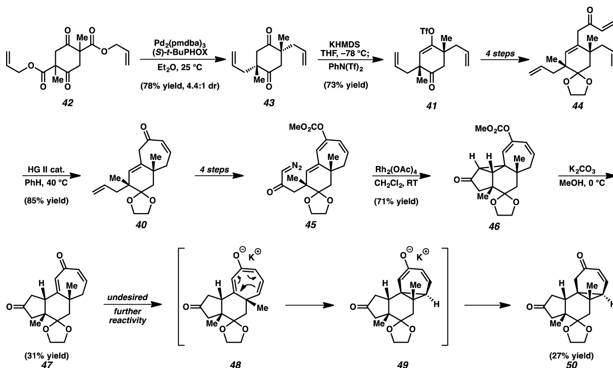
Scheme 10. Synthesis of the gagunin core.
