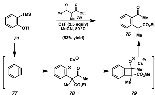
Scheme 19. Unexpected aryne C–C insertion and mechanistic proposal.
