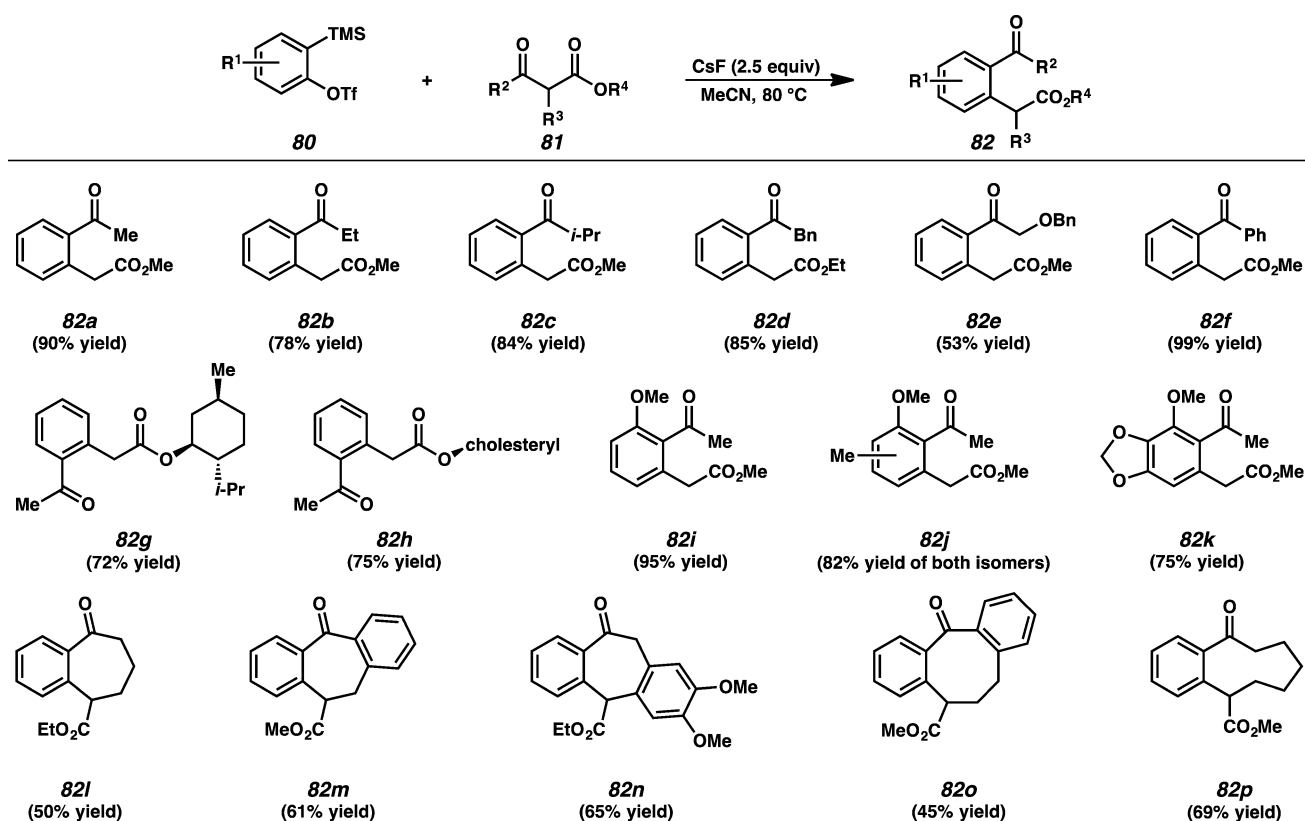
Scheme 20. Scope of the acyl-alkylation of arynes.
