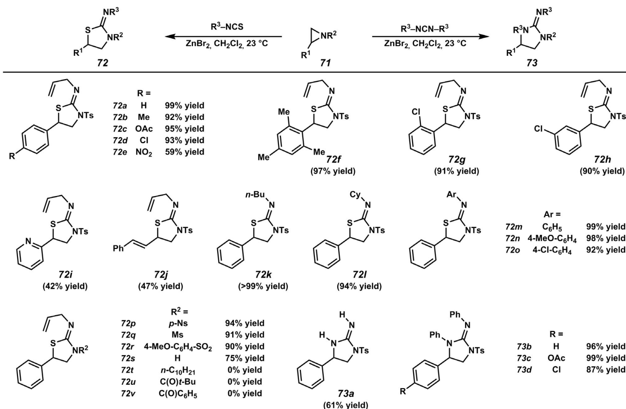
Scheme 17. Selected scope of cycloadditions of activated aziridines with heterocumulenes.
