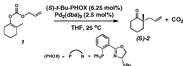
Scheme 2. The Enantioselective Tsuji Allylation Mechanism Studied in This Work 10
