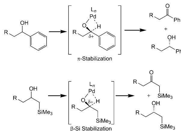
Scheme 5. Stabilization of the \beta -hydride elimination transition state by resonance and a \beta -silicon.
